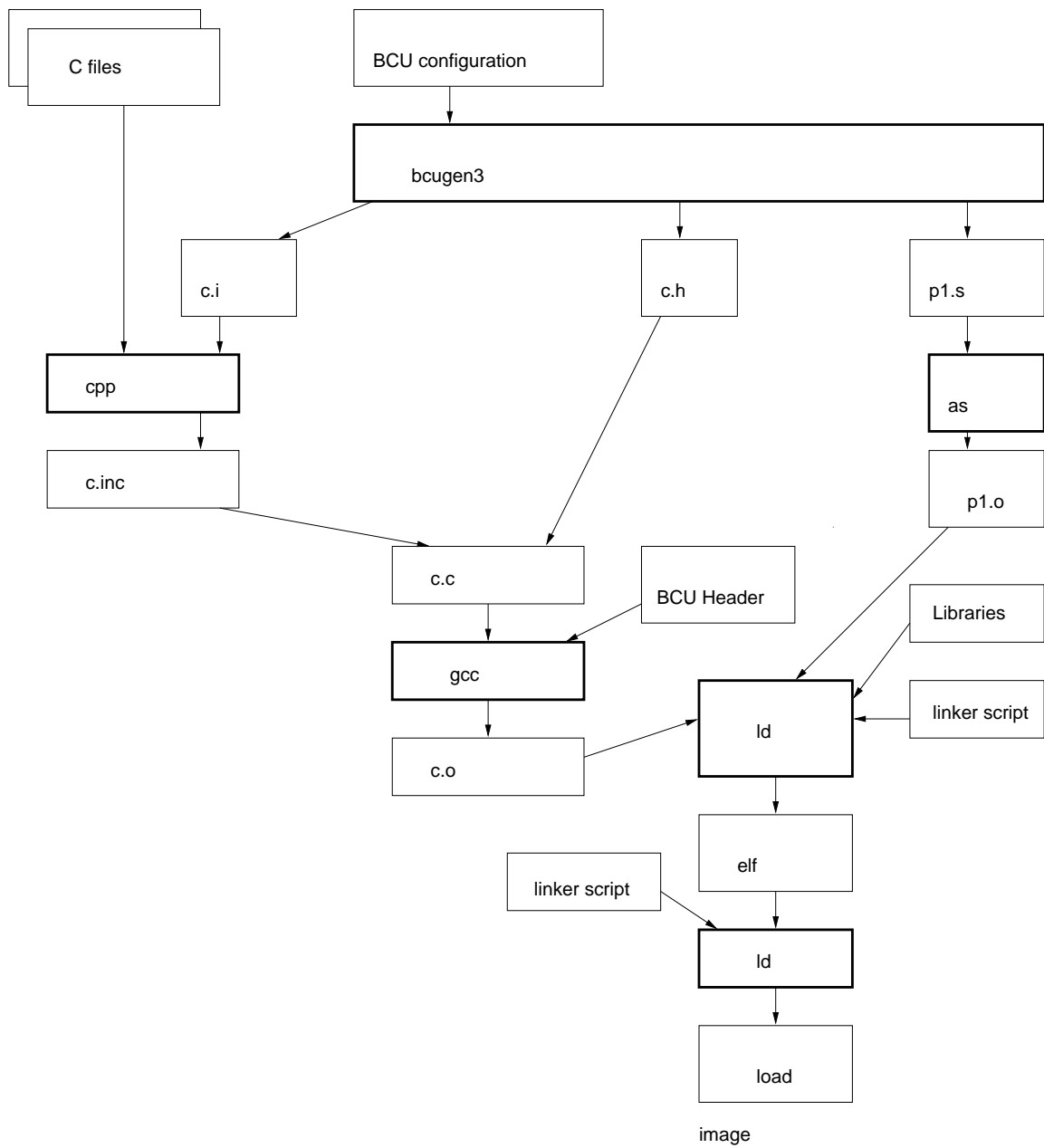
Figure 6.3.: build.dev operational sequence and data flow
